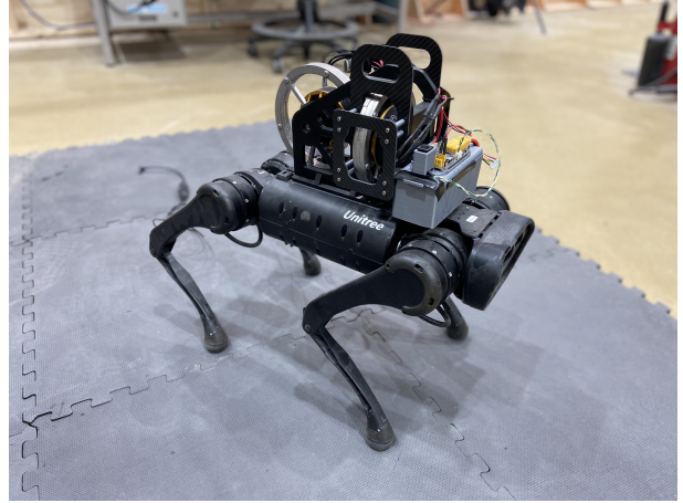
Fig. 1: The Unitree A1 Quadruped mounted with our custom-made reaction wheel module.
