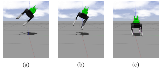
Fig. 4: A drop test sequence where the robot reorients itself with the torques from the x axis reaction wheel.
