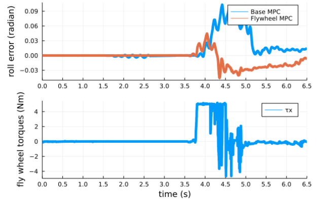
Fig. 2: Robot roll error responses to a 350N impulse on the body frame y-axis at t = 3.6 seconds. The top graph illustrated the roll error trajectory with respect to time for the base MPC controller and the reaction wheel assisted controller. The bottom graph plots the torque exerted by the x-axis reaction wheel during the experiment.
