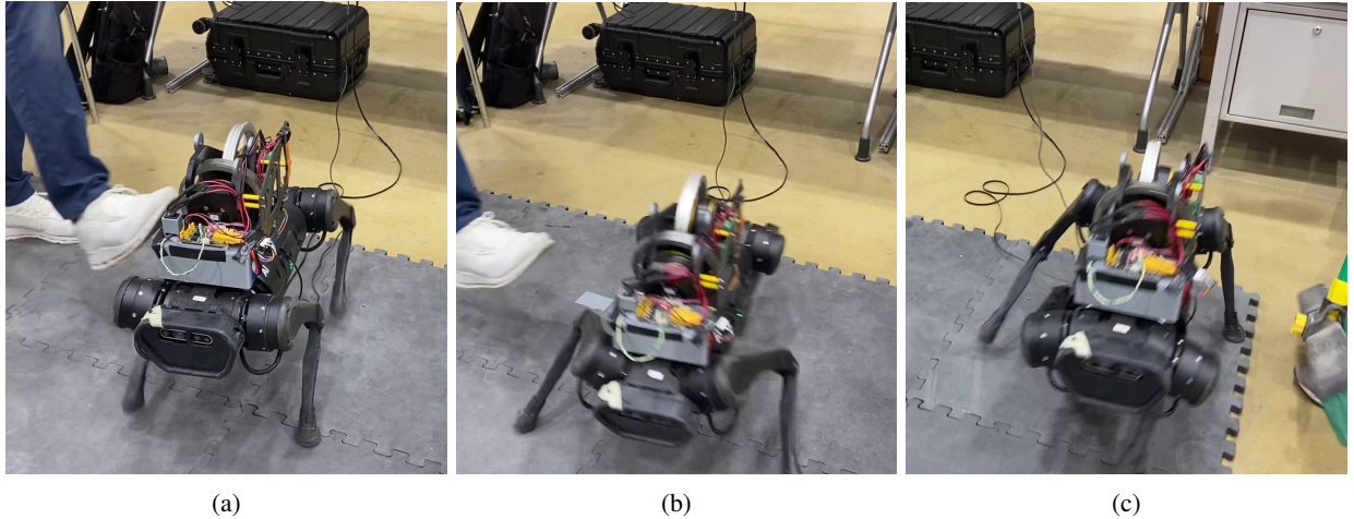
Fig. 3: Hardware impulse test where we provide a impulse force on the robot during locomotion with a kick. Figure 3a shows the robot in stable trotting phase when the impulse is applied. Figure 3b shows the robot losing balance on the footholds while maintaining a stable attitude as it eventually recovers from the impulse in Figure 3c.
